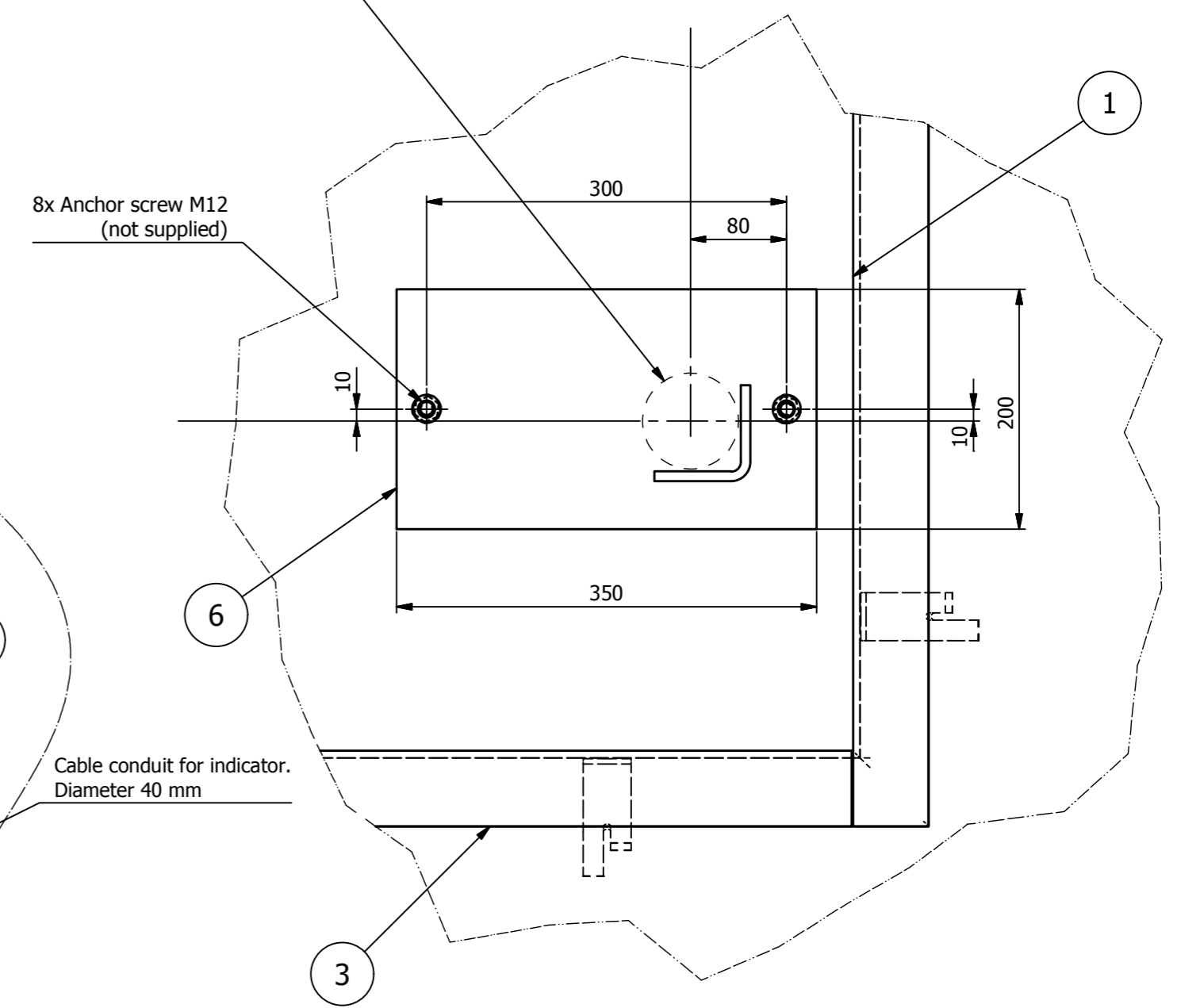
Detail C (1 : 5)
